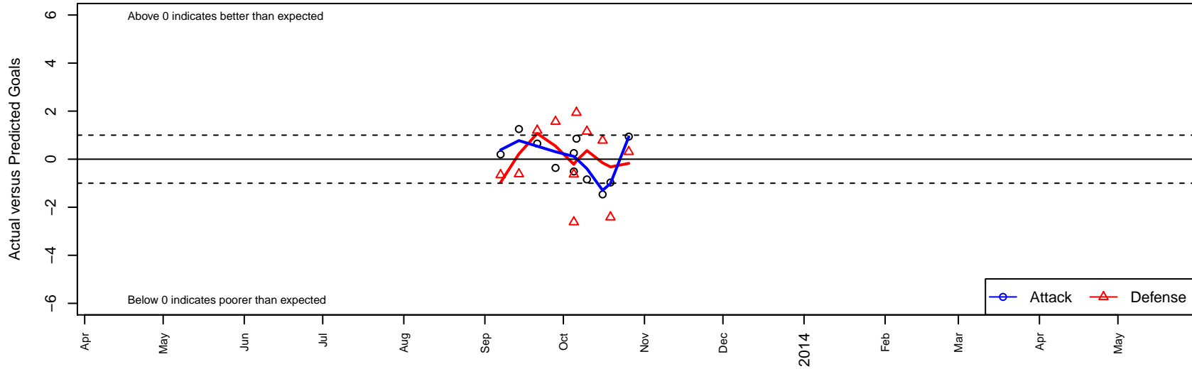
Idaho Inferno B01 Dots are actual minus expected GF (blue circles) and GA (red triangles). Blue line is smoothed change in attack strength. Red is smoothed change in defense strength.
